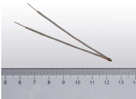
Figure 1.2 Physical Photo of the ATH100K1R25T70
