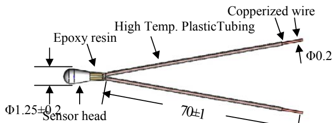
Figure 2. Side View of ATH100K1R25T70S
